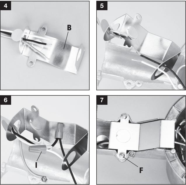
Conduit and Junction Box not shown
