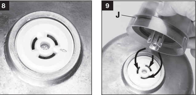
Conduit and Junction Box not shown
